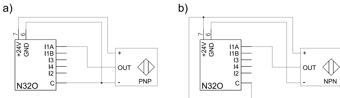
Fig. 6: Connection of the N32O meter.
