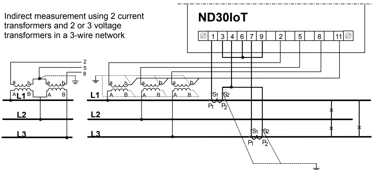
Fig. 7. Meter connections of input signals in a 3-phase 3-wire network
