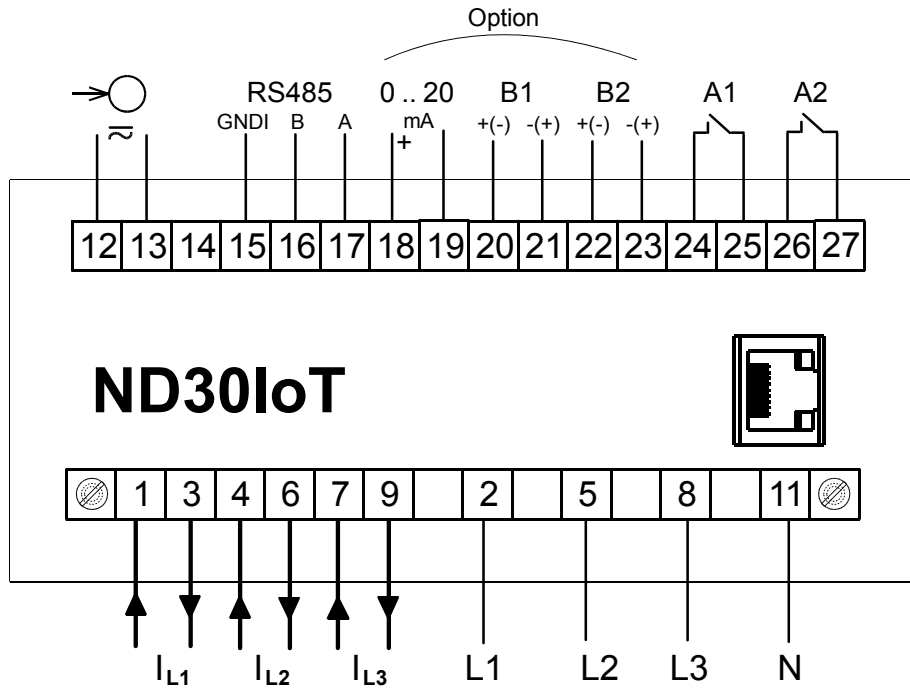
Fig. 4. Meter connections
